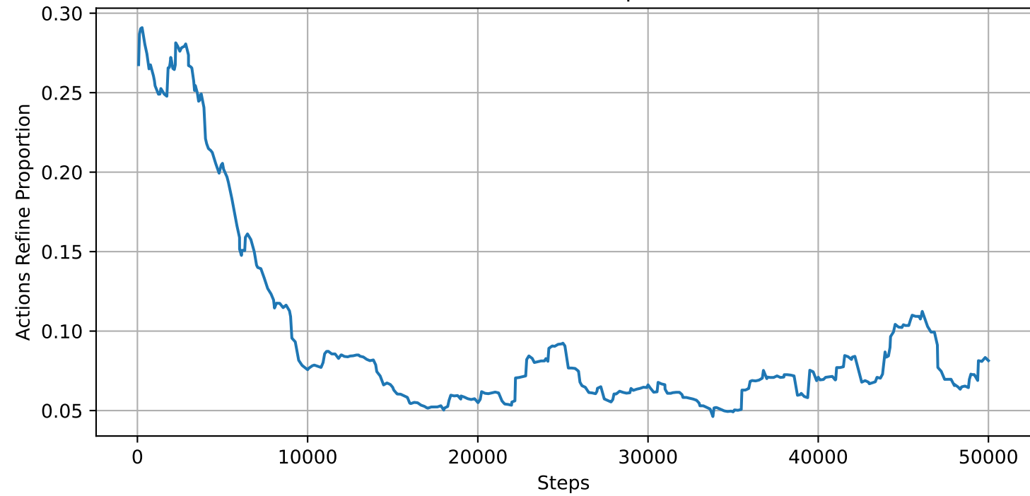
Actions Refine Proportion
