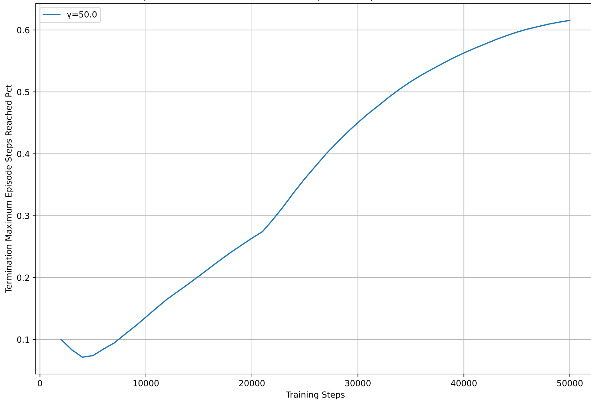
Comparison of Termination Maximum Episode Steps Reached Pct Across Runs
