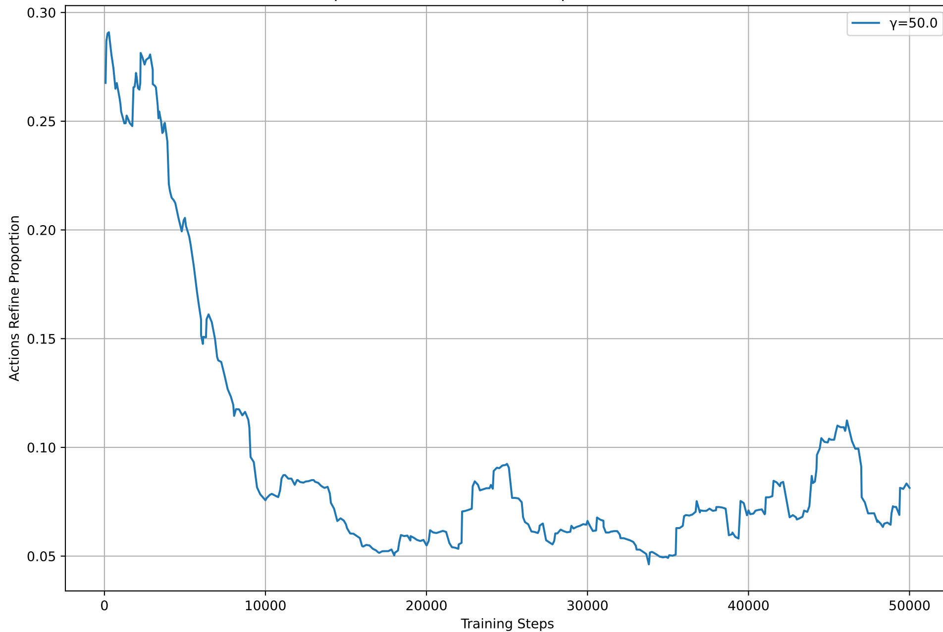
Comparison of Actions Refine Proportion Across Runs
