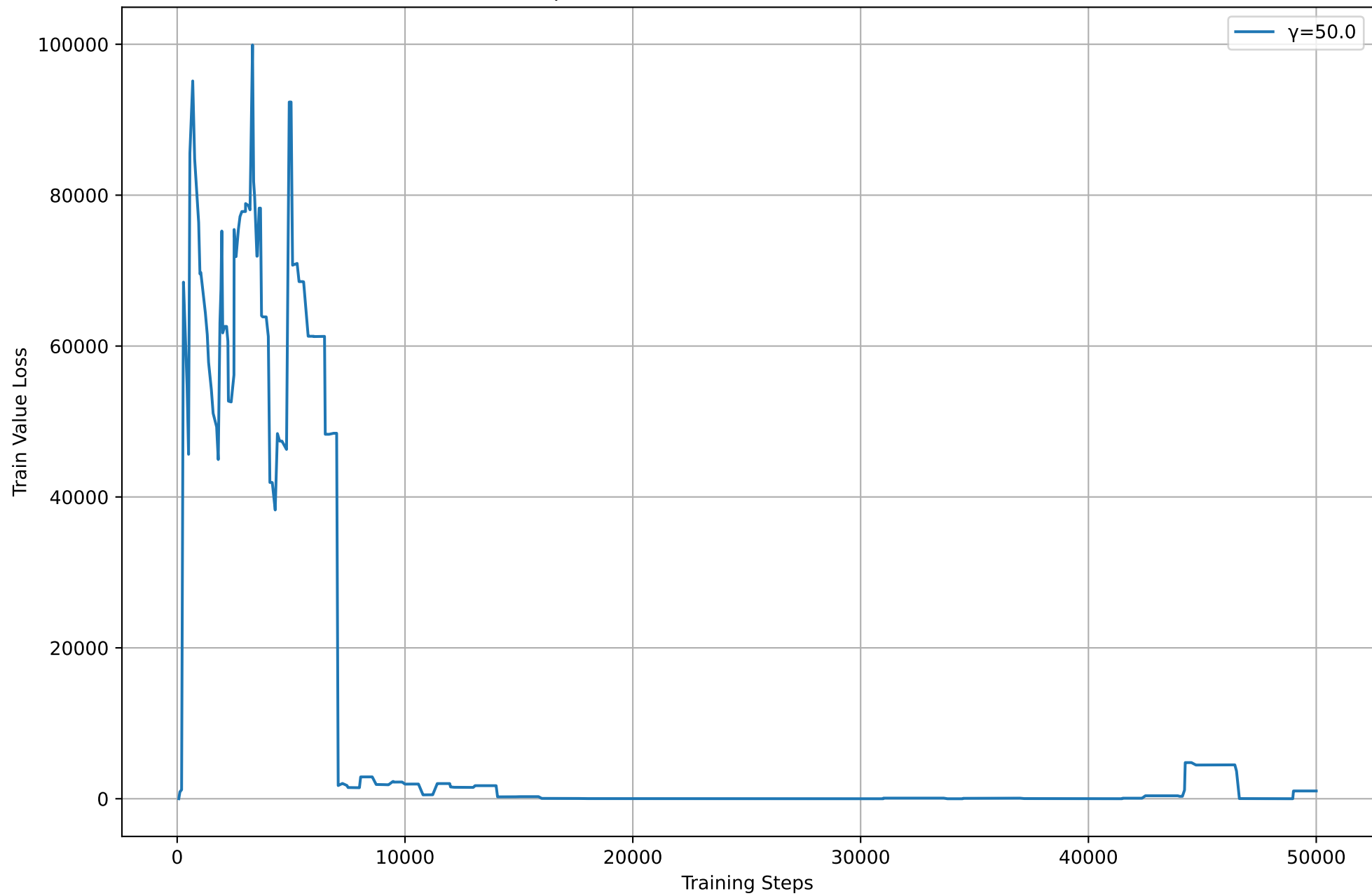
Comparison of Train Value Loss Across Runs
