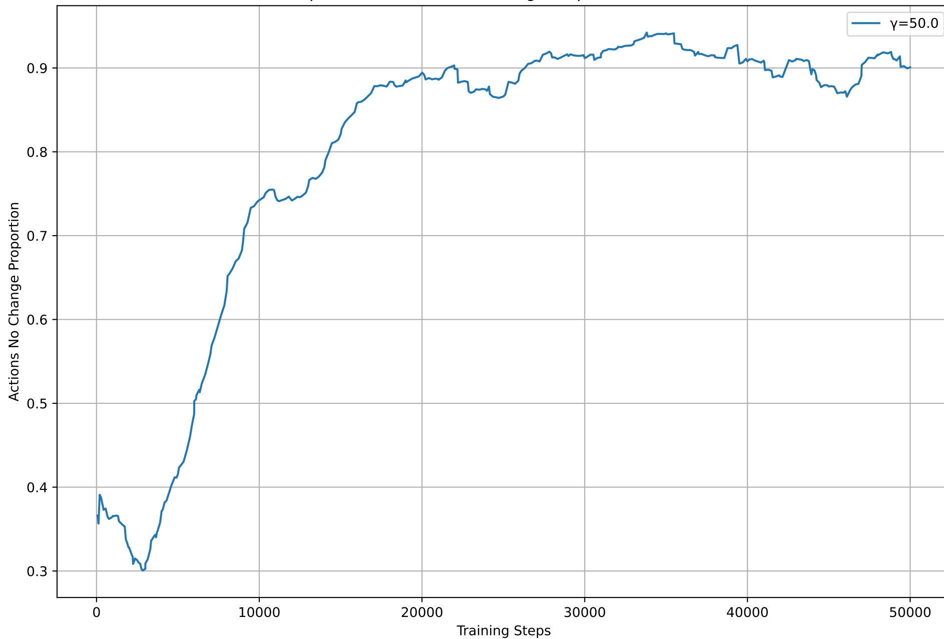
Comparison of Actions No Change Proportion Across Runs
