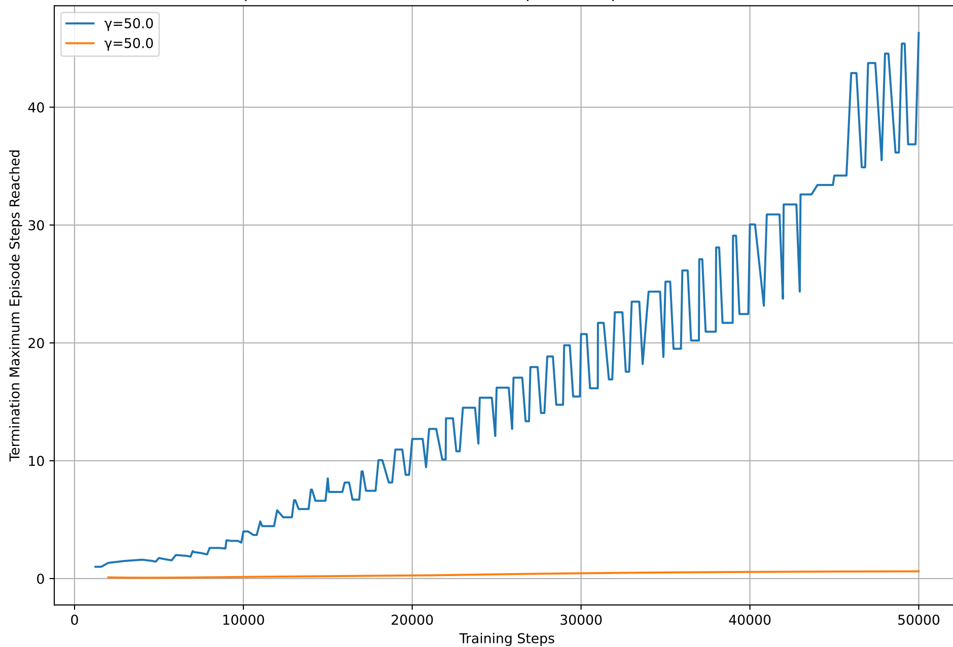
Comparison of Termination Maximum Episode Steps Reached Across Runs
