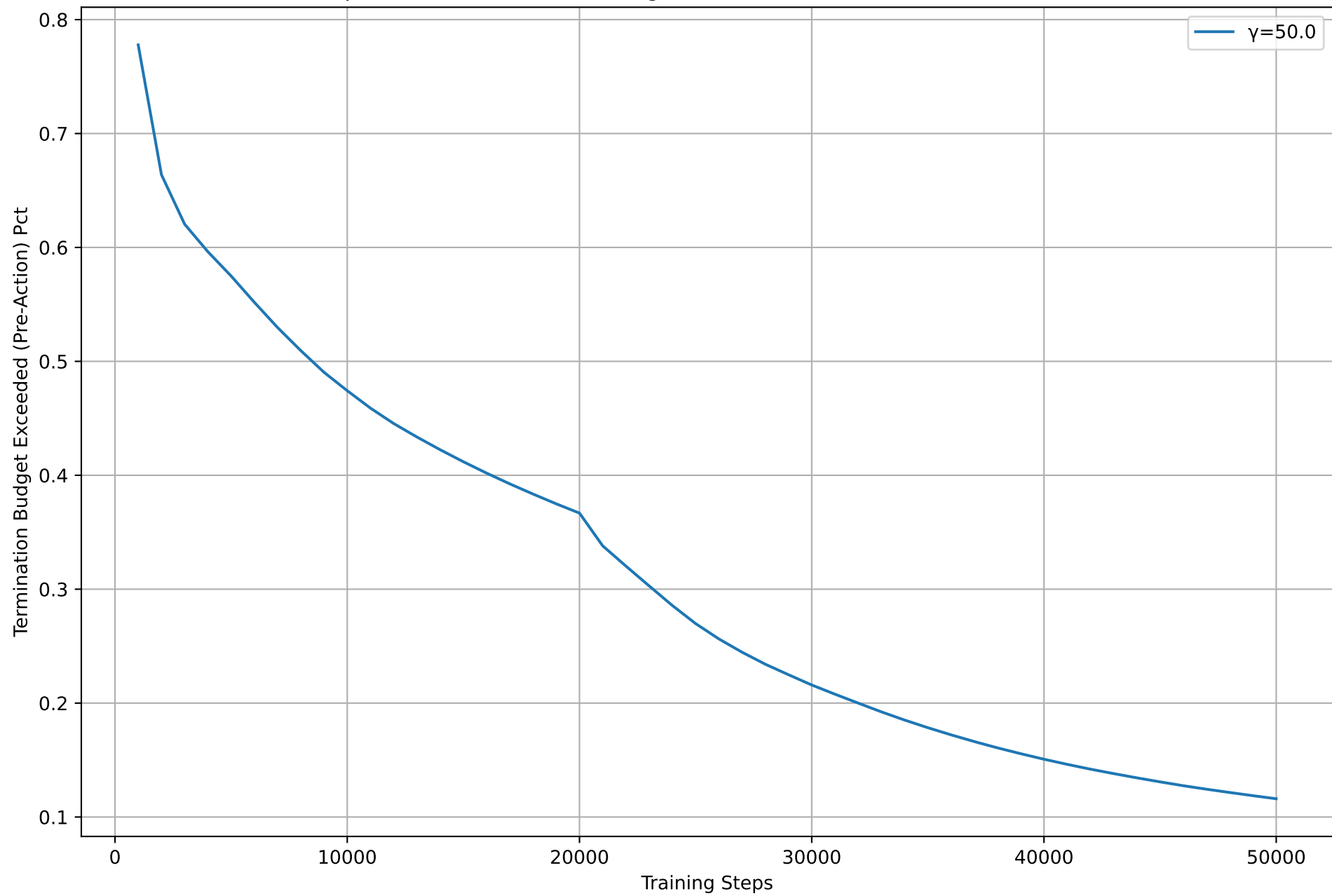
Comparison of Termination Budget Exceeded (Pre-Action) Pct Across Runs
