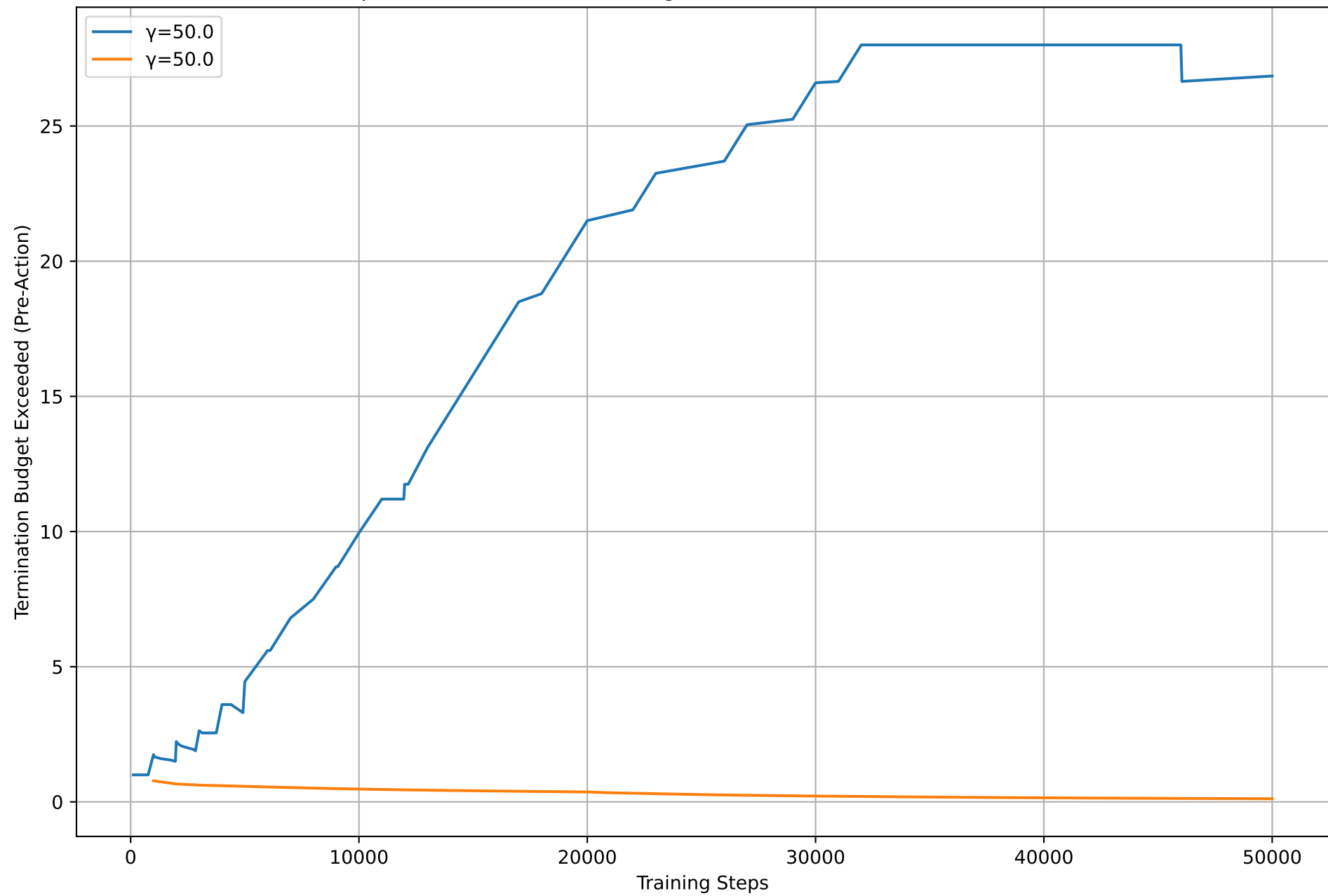
Comparison of Termination Budget Exceeded (Pre-Action) Across Runs
