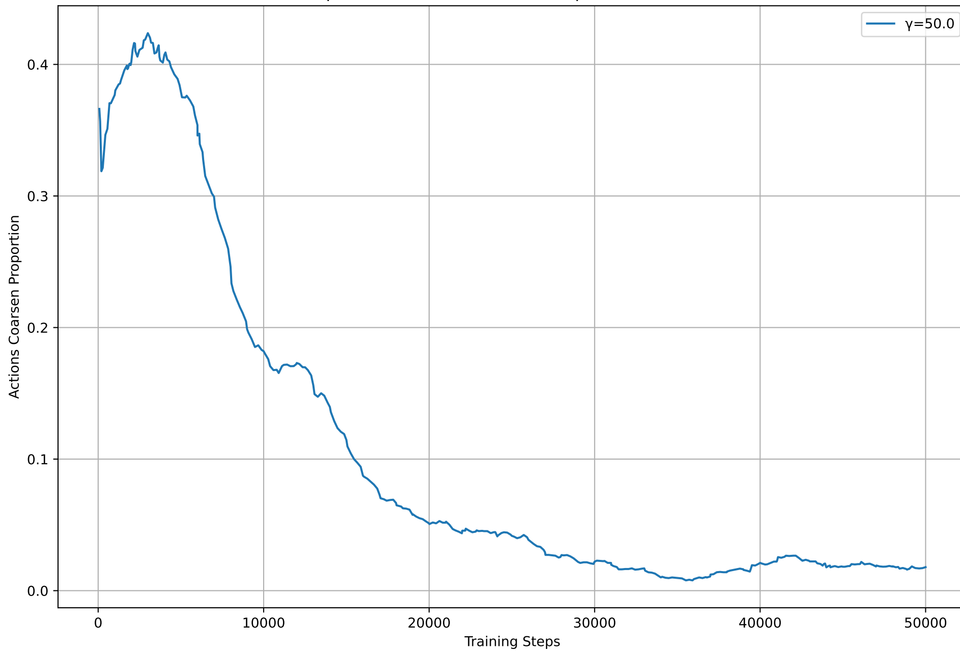
Comparison of Actions Coarsen Proportion Across Runs
