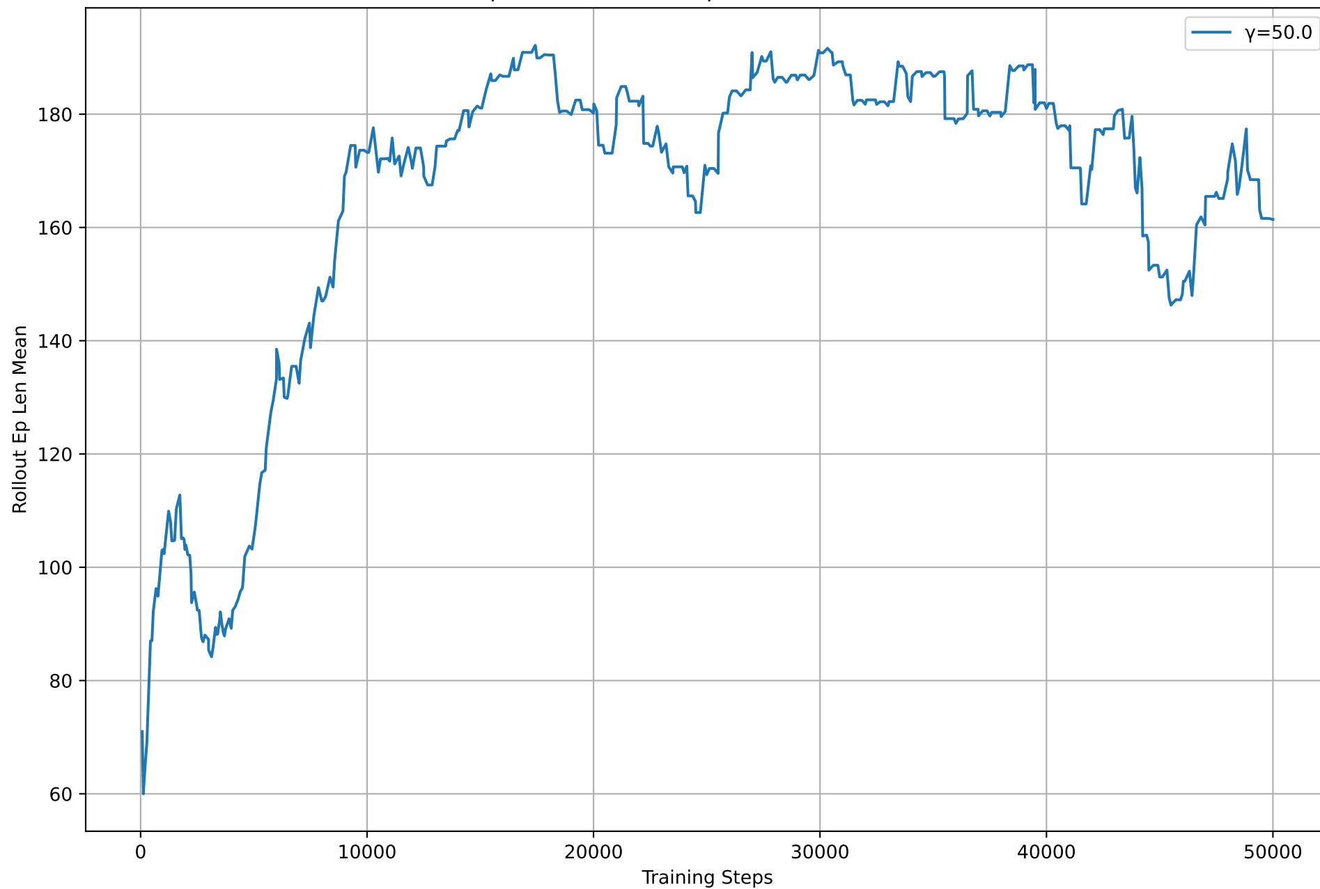
Comparison of Rollout Ep Len Mean Across Runs
