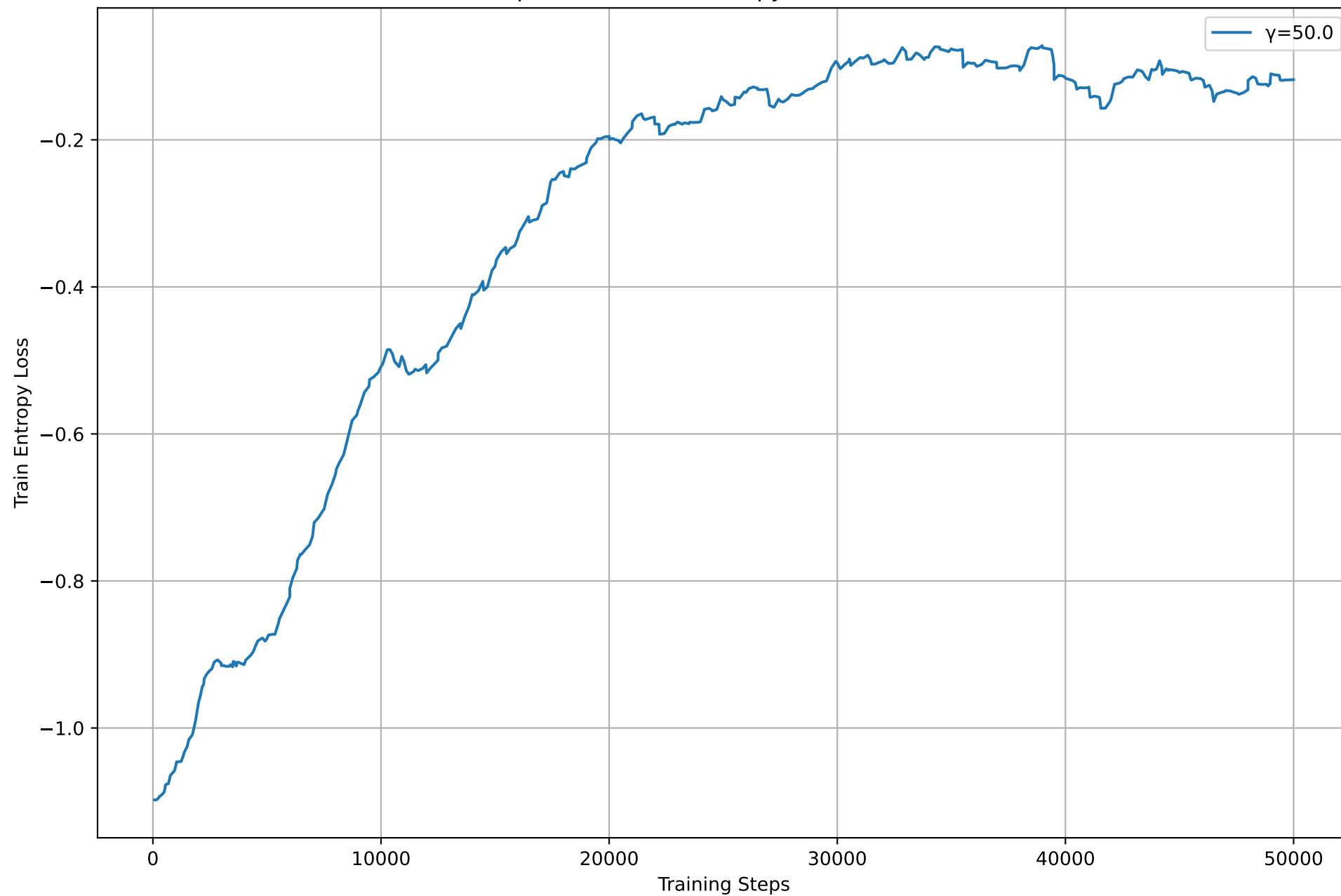
Comparison of Train Entropy Loss Across Runs
