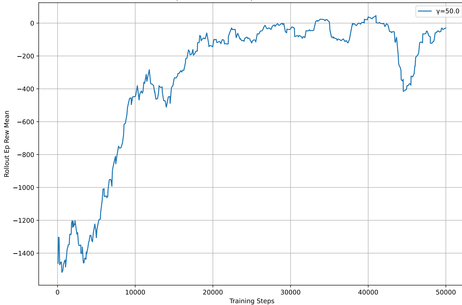
Comparison of Rollout Ep Rew Mean Across Runs
