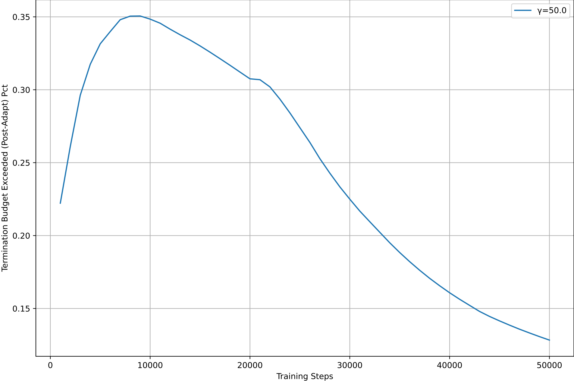
Comparison of Termination Budget Exceeded (Post-Adapt) Pct Across Runs
