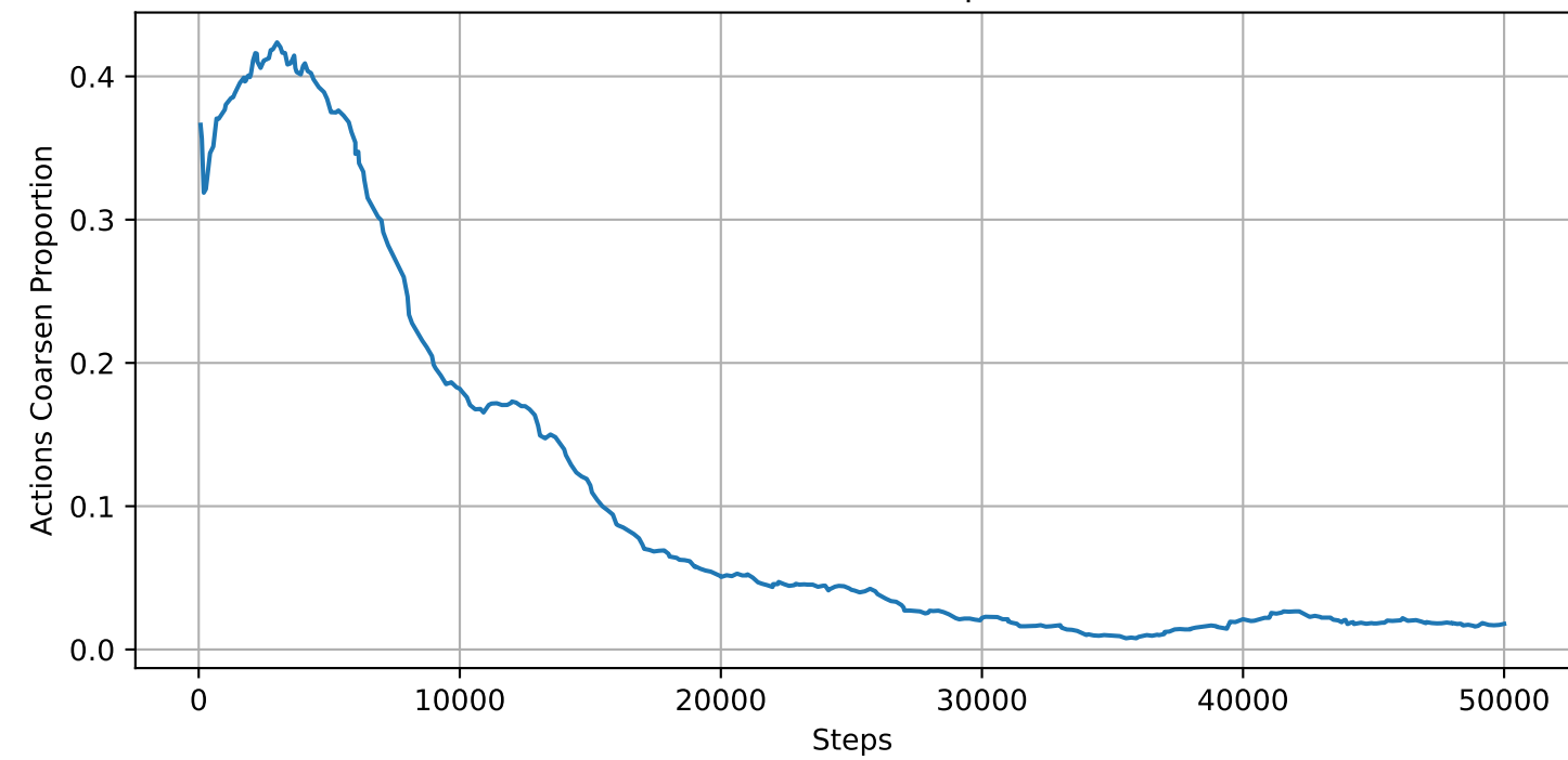
Actions Coarsen Proportion
